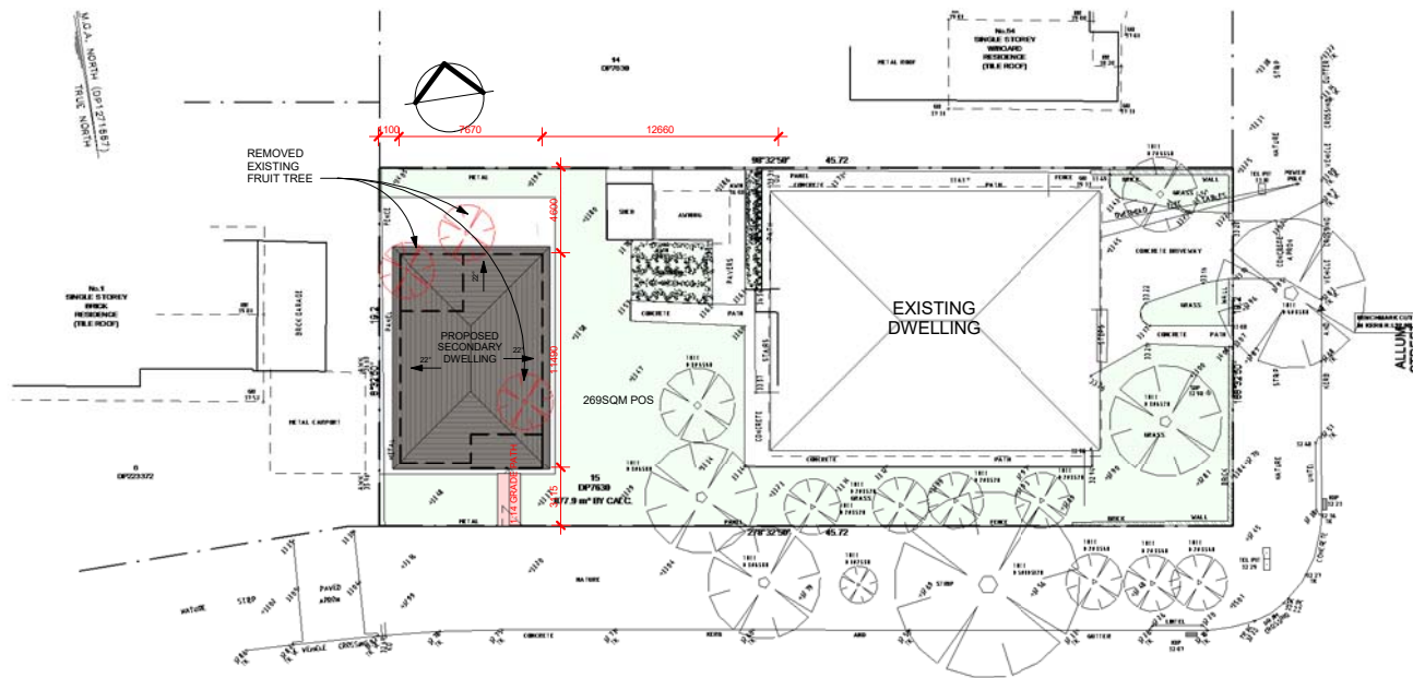
1 00 SITE PLAN / ROOF PLAN (GRANNY FLAT) - Dependent 1 1:200
