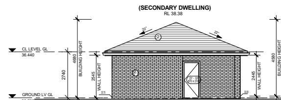
3 NORTH ELEVATION - Dependent 1 1:100
