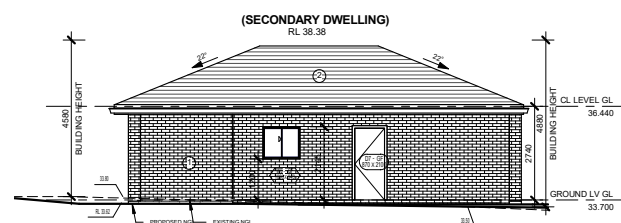
5 WEST ELEVATION - Dependent 1 1:100
