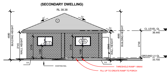
4 SOUTH ELEVATION - Dependent 1 1:100
